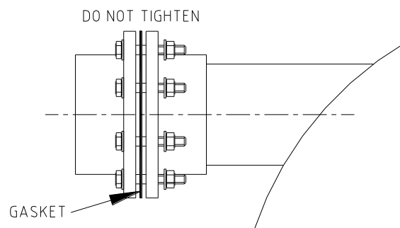
Figure 2 : Initial connection to the filter's flanges
