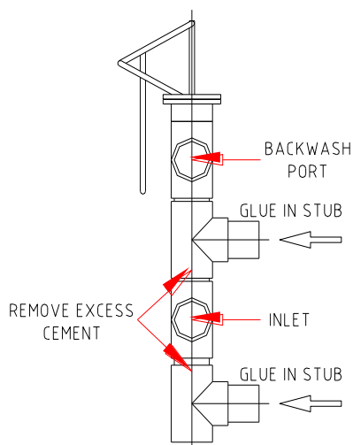
Figure 3 : Valve Connections
