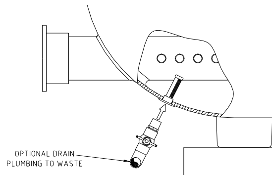
Figure 6: Screened Drain Valve (with 40BSP male thread)
