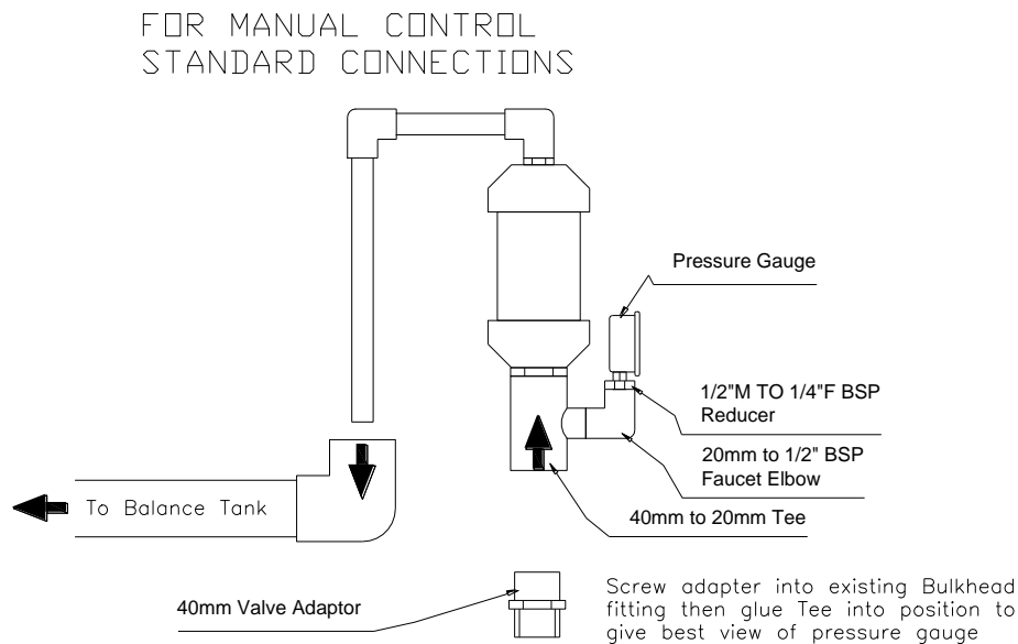
Figure 8 – Typical Installation Chadson Kinetic Valve (Type A)
