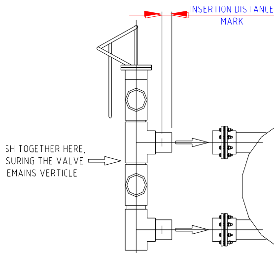
Figure 4 : Fitting to Filter
