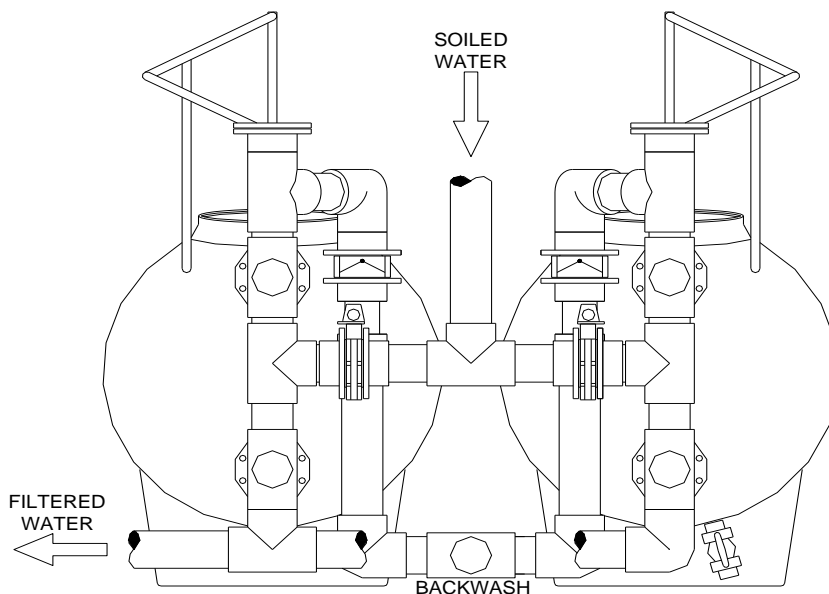
Figure 5 – Typical Multiport Valve Connections
